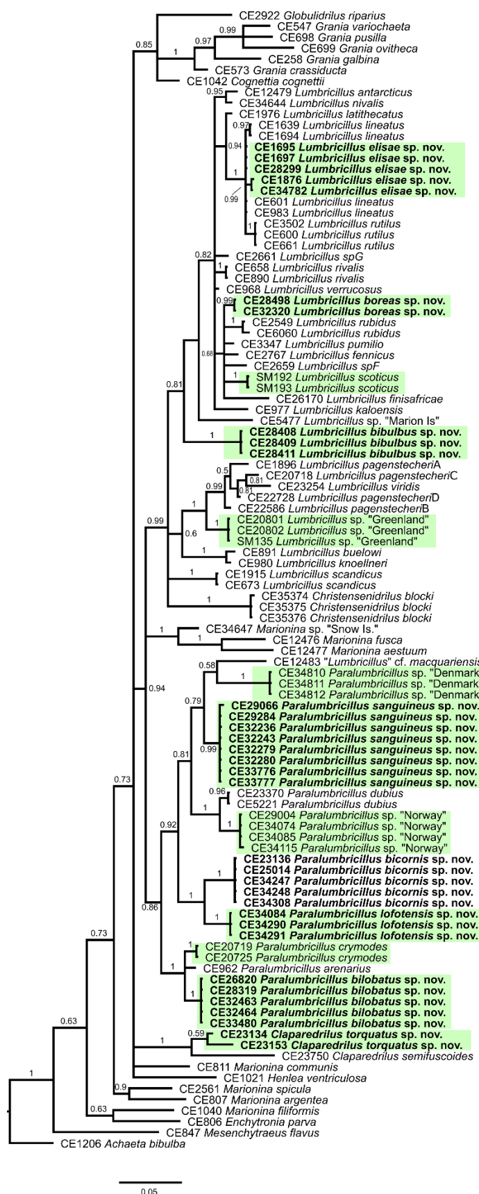
Figure S3. Majority-rule consensus tree for H3 estimated with Bayesian inference. Specimens marked in green are new to this study. Support values are posterior probabilities. Scale bar represents the estimated number of substitutions per site.
