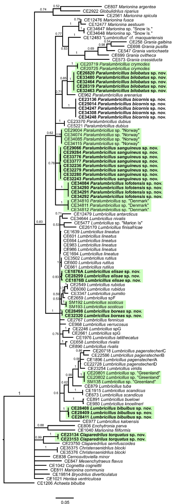
Figure S2. Majority-rule consensus tree for ITS2 estimated with Bayesian inference. Specimens marked in green are new to this study. Support values are posterior probabilities. Scale bar represents the estimated number of substitutions per site.
