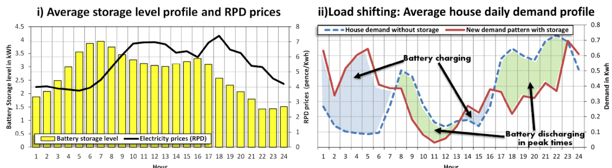
Figure 5.1: Example of a prosumer exposed to hourly time-of-use price (ToU) price variations [79]
