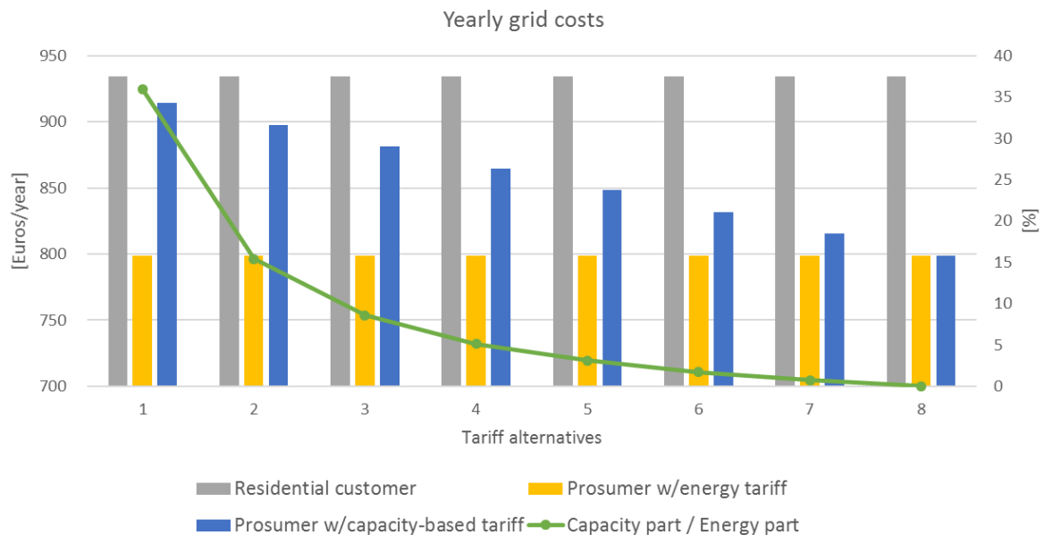
Figure 4.2: Consequences for prosumer when changing different parts in the grid tariff [39]
