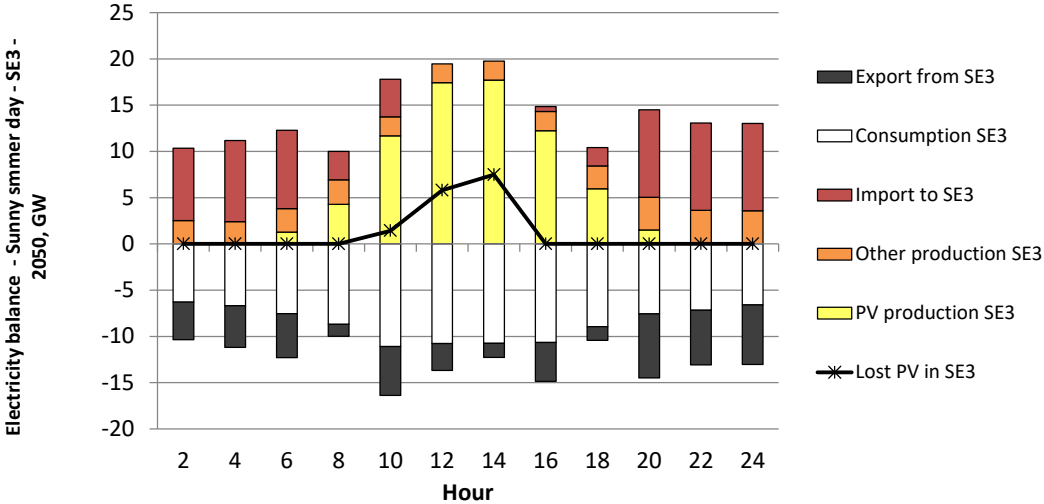
Figure 6.3: The electricity balance of a sunny summer day in 2050 for PRO+ in the SE3 spot price region in Stockholm
