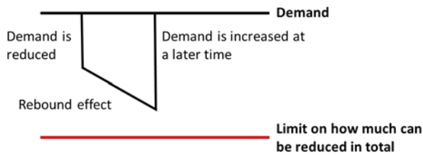
Figure 6.5: Concept of shiftable DR
