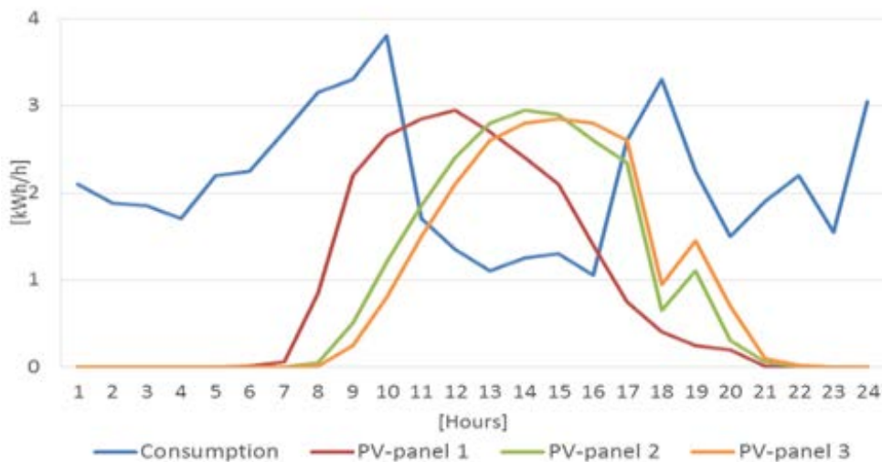
Figure 5.2: Changes in feed-in of electricity as a consequence of PV panel orientation
