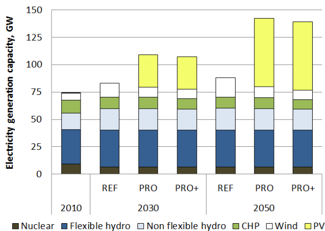
Figure 6.2: Electric generation capacity in Scandinavia by technology, for REFerence (REF), PROsumer (PRO) and PROsumer plus (PRO+) in 2010, 2030 and 2050
