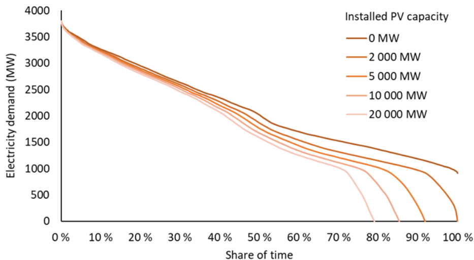
Figure 6.1: Load duration curve of the electricity demand in the region of Oslo with different levels of PV capacity
