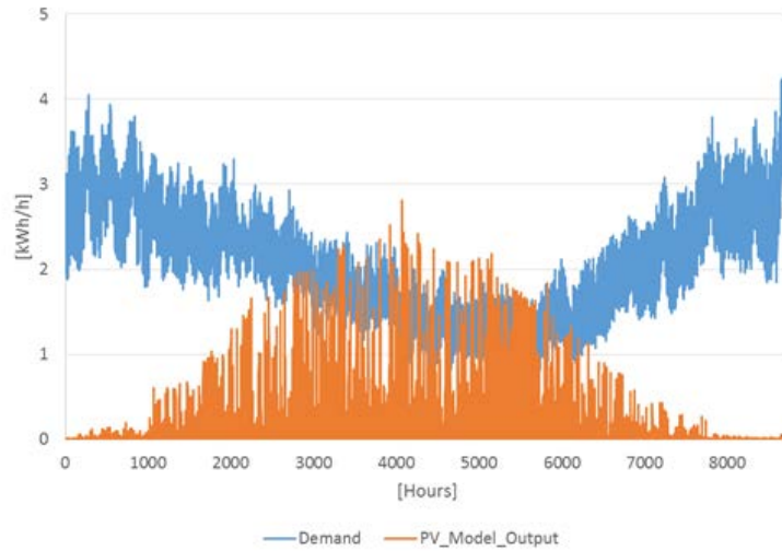
Figure 4.1: Load curve for typical residential customer and modelled PV generation [39]
