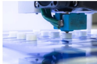
Figure 2: Production of personalised Printlets™ directly onto blister packaging using the M3DIMAKER™ system.
