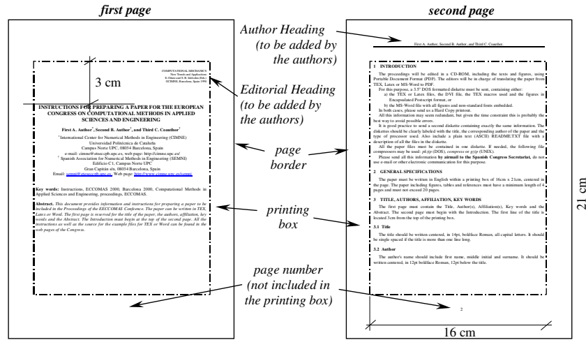
Figure 1: Page layout
