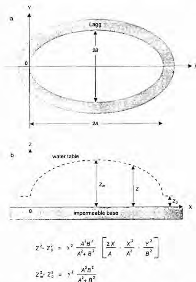
Fig. 3. Dimensions of the groundwater mound model on an elliptic base; a: plan view, b: profile along major axis.
