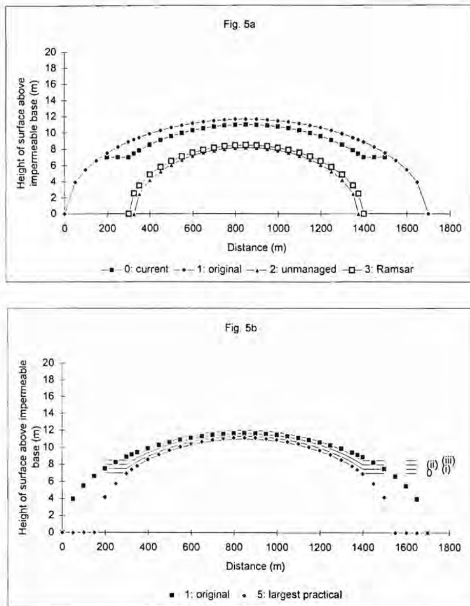
Fig. 5. Comparison of major-axis ( Y = 0 ; see Fig. 3) profiles of groundwater mound models representing existing and hypothetical management scenarios for Puergschachenmoos. (a) supposed original mire, current situation and unmanaged scenarios 2 and 3. (b) points: supposed original mire and scenario 5; lines: current situation (0) and scenarios with management to raise marginal water levels by (i) 0.5 m, (ii) 1 m and (iii) 1.5 m. See text for further details of scenarios.
