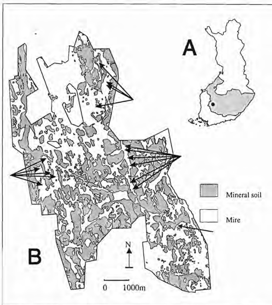
Fig. 1. A. The location of the Seitsemien National Park. The eccentric bog zone (according to Ruuhijärvi 1988) is shaded. B. Mires in the Seitsemien National Park. Arrows show the location of study sites.
